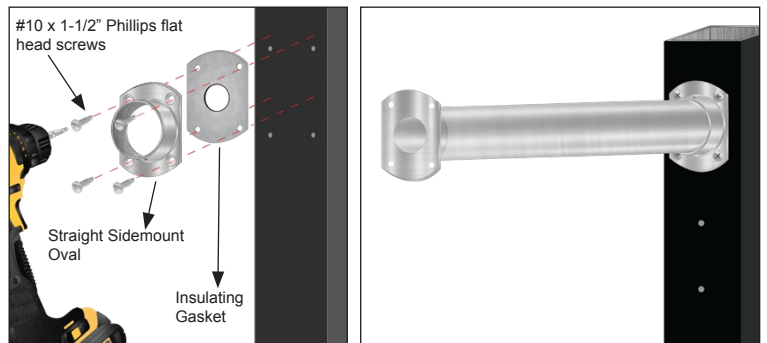
Figure F. (LEFT) Install using four (4) #10 x 1-1/2" Phillips flat head screws.
