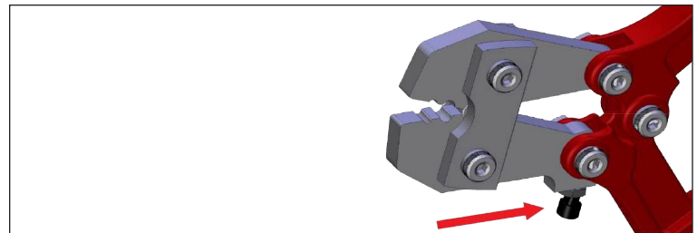
Figure F. To increase crimping force, loosen lock nut and rotate the adjustment bolt on the tool clockwise. Tighten the lock nut once the desired adjustment is achieved.
