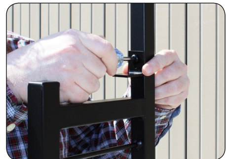
Figure C. Install the “L” brackets using the provided machine screws and nuts. Do not fully tighten the brackets to the frame.
