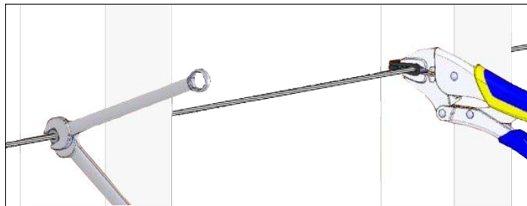
Figure Q. Use a cable grip pad with vice grips to hold the cable tight.
