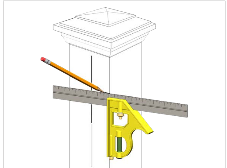
Figure V. Use a square and tape measure to mark the center of your posts.
