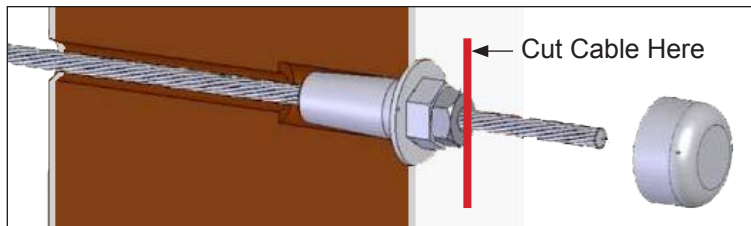
Figure P. Put the cable through the flush fitting. Push it against the back of the post and pull the cable tight and cut.
