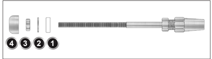
Figure AI. Deluxe Cover Nut Set assembly diagram - 1) Plastic Washer, 2) Stainless Steel Washer, 3) Stainless Steel Nut & 4) Stainless Steel Deluxe Cover. RailEasy Stud Assembly not included.
