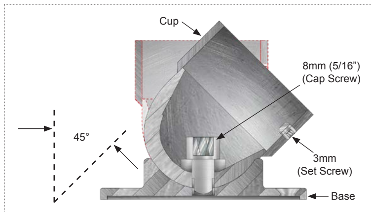
Figure X. Tighten down the screw of the Rail Side Mount Adjustable 2.
