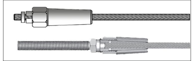
Figure AC. Cutaway view of the RailEasy Tensioner
