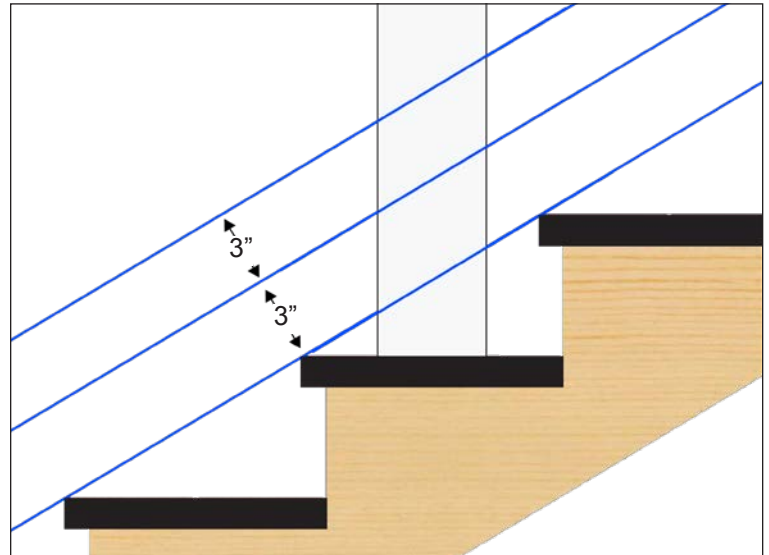
Figure Z. Measure perpendicularly from the chalk line to find the center line of your cables.
