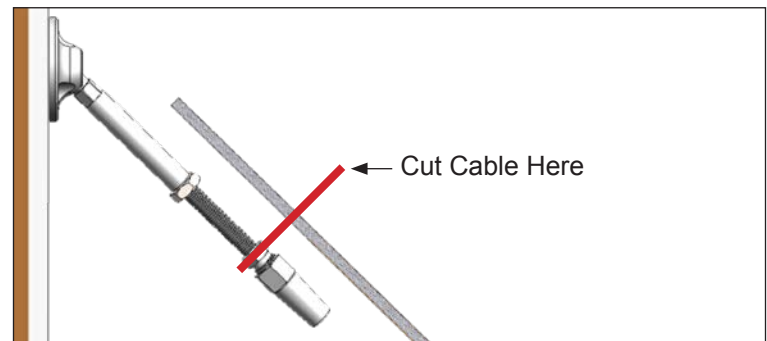
Figure AD. Pull the cable tight to the tensioner and cut it.
