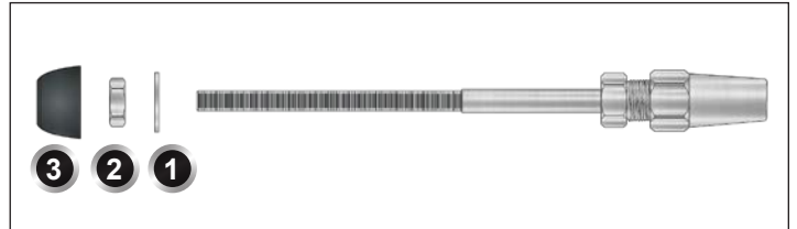
Figure AJ. HandiSwage Cover Nut Set assembly diagram - 1) Stainless Steel Washer 2) Stainless Steel Nut & 3) HandiSwage Cover. RailEasy Stud Assembly not included.
