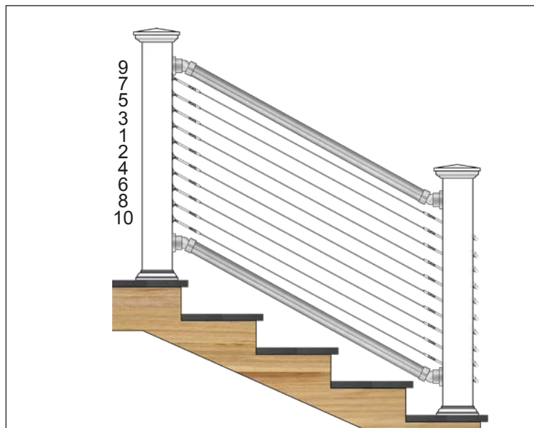
Figure AG. Tensioning Diagram - Begin with the center run of cable and alternate working above and below until cables are tight.
