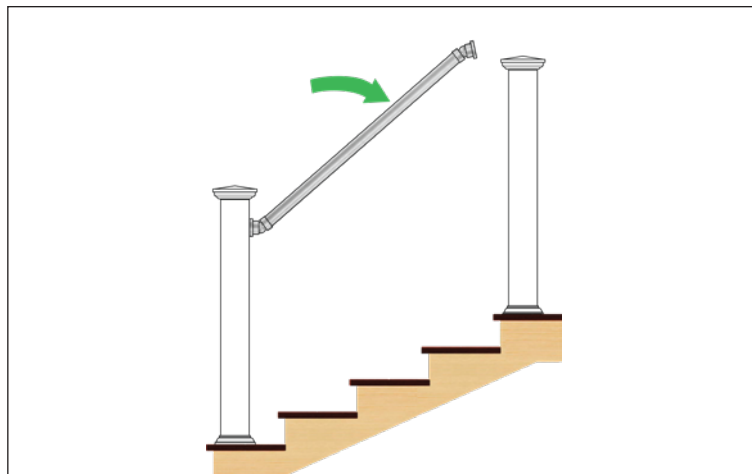
Figure W. Rotate the railing down and line up the top holes with the pre-drilled holes from the previous step.
