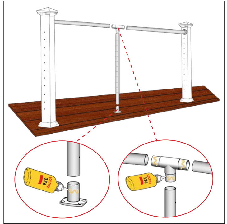
Figure AM. Apply a thin bead of Loctite 326 brand adhesive to the post base and rail tee when you are comfortable that the dry-fit sections are correct.
