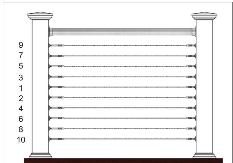
Figure T. Tensioning Diagram - Begin with the center run of cable and alternate working above and below until cables are tight.
