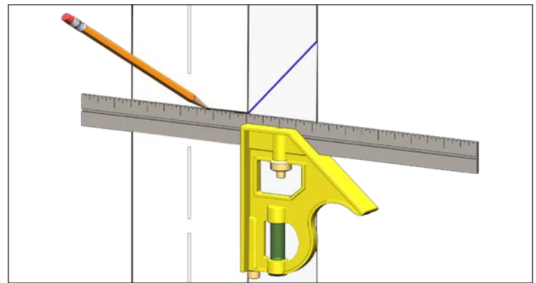
Figure AA. Using a carpenter's square, transfer the chalk line to the inside face of the post. The intersection of this line and the vertical will mark your center.
