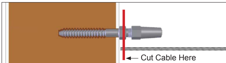
Figure S. Pull the cable tight to the lag stud end and cut it.
