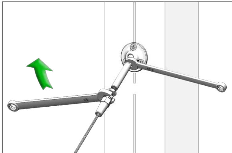
Figure AF. Hold the tensioner terminal still with a 3/8" wrench and using a 5/16" open wrench, rotate tensioner body to tension.
