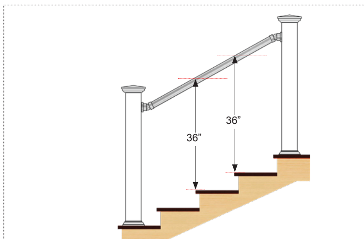
Figure Y. Measure vertically 36" from the edge of the nosing of the stair. This is the height of the top of the rail.
