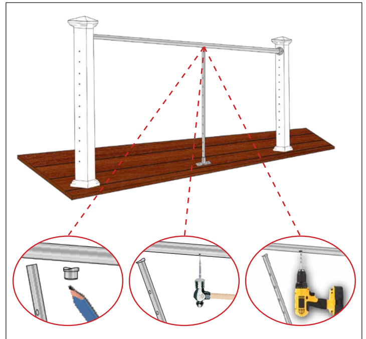
Figure AN. With base and top plate positioned as desired mark the screw holes (top and bottom), remove stabilizer, tap and drill pilot holes.
